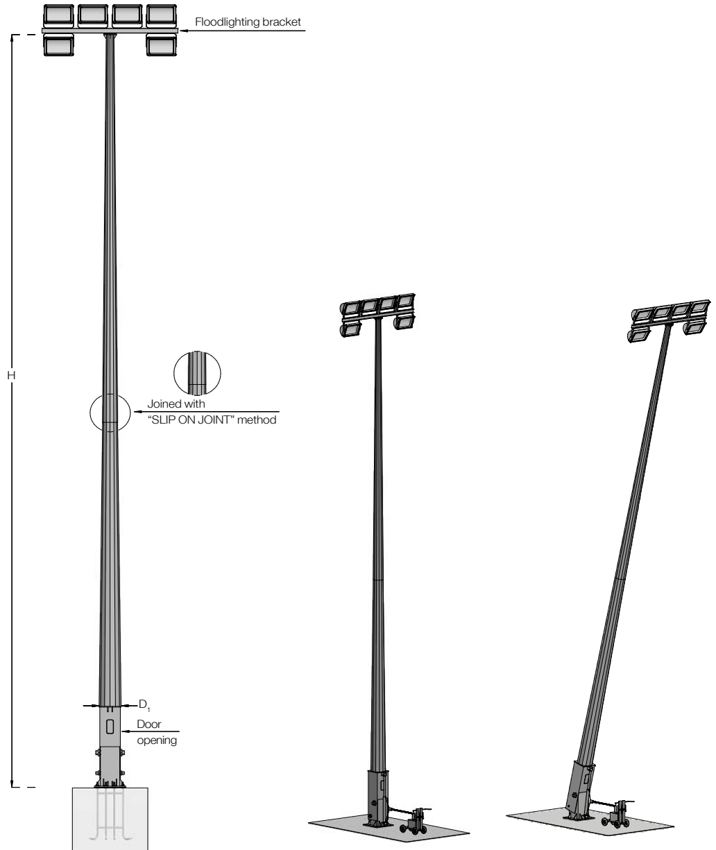
Mast drawing model
